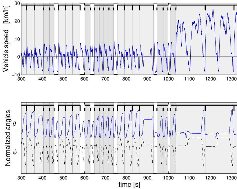
Figure 9: A cycle-partitioned dataset. White = No cycle, Light gray = Loading cycle, Dark gray = cleaning cycle
