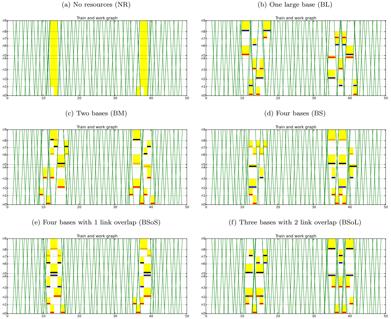
Figure 4: Solutions to instance L6
