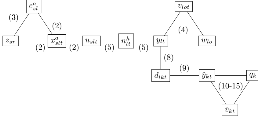
Figure 2: Variable and constraint graph — resource model
