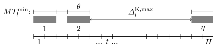
Figure B.1: Calculation of MT_l^{\min} and \Delta_l^{K, \max}
