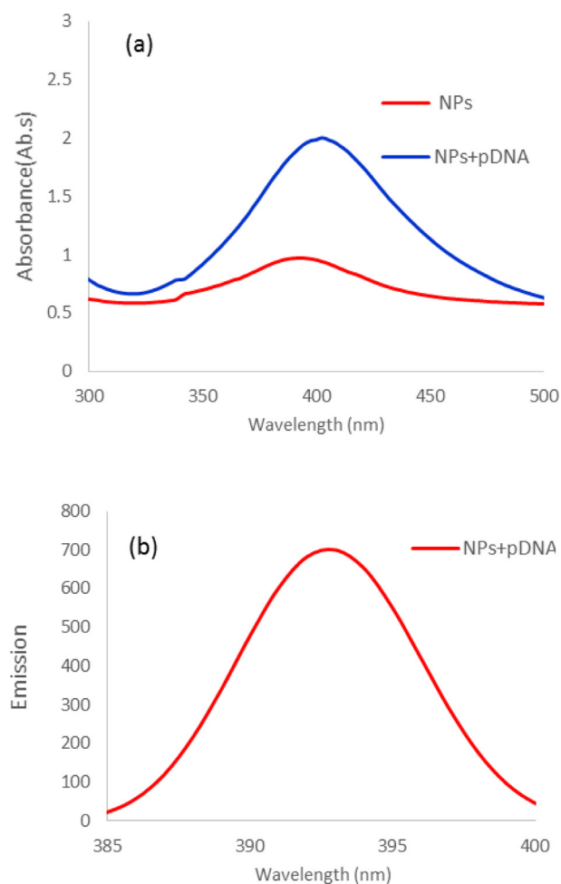
Figure 1. (a) Uv/Vis absorbance spectrum of Citrate-AgNPs and Citrate AgNPs after conjugation with pDNA (b) Fluorescence emission spectrum of Citrate AgNPs after conjugation with pDNA.
