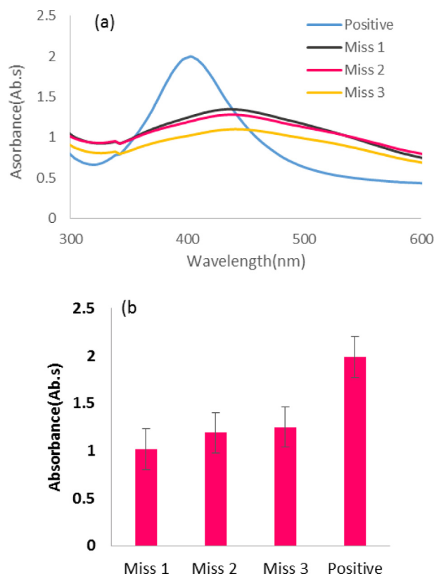
Figure 5. (a) UV-Vis absorbance spectrum of cDNA hybridization with mismatch 1, mismatch 2 and mismatch 3. (b) Histogram of cDNA hybridization with mismatch 1 (5′CCGACACAGCGATCTGCTTACGAGAT 3′), mismatch 2 (5′CCGACACAGCGATCTGCTTACGAGAT 3′) and mismatch 3 (5′GTGACACAGCGATCTGCTTACGAGAT 3′) and positive sequences.
