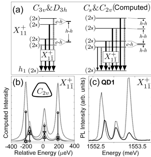
FIG. 4. (a) Polarized radiative decay paths of the positive trion X_{11}^+ for the ideal case C_{3v} (left) and the asymmetric case C_s (right). The numerical model yield dark transitions indicated by thin lines and small arrows. Black solid lines indicate both x - and y -polarized light. Dotted lines indicate z -polarized light. (b) Computed exciton spectra of X_{11}^+ (see caption of Fig. 3). (c) Close-up PL of X_{11}^+ .
