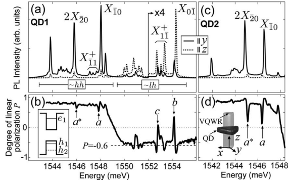
FIG. 2. (a) and (c) Polarized PL spectra of two QDs and (b) and (d) the corresponding degree of linear polarization. The PL is recorded for polarization vectors perpendicular (solid lines) and parallel (dotted lines) to the growth direction z . The insets illustrate schematic diagrams of (b) single particle energy levels and (d) the QD geometry.
