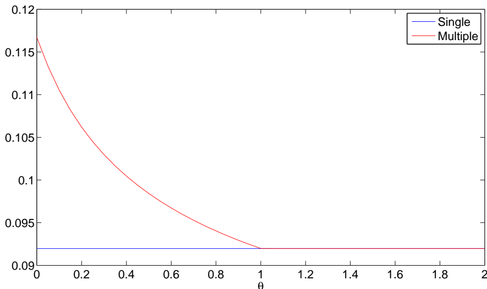
Figure 13: l_\infty -error of the single and multi domain operator as a function of \theta using 33 and 34 grid points respectively.
