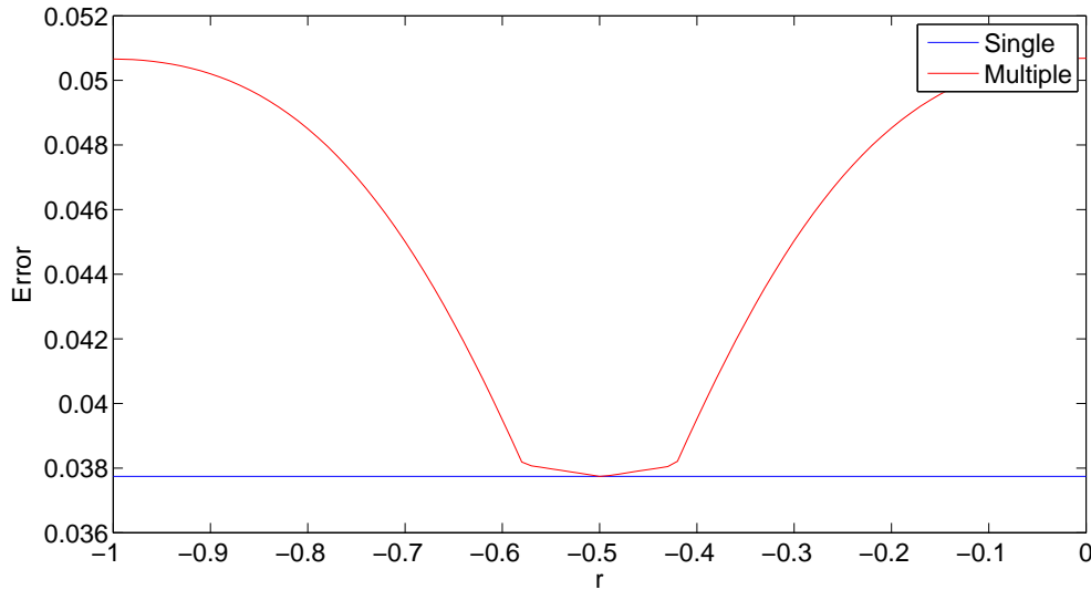
Figure 9: l_\infty -error at t = \frac{\pi}{2} as a function of r with 33 grid points for the single domain and 34 for the multi domain.
