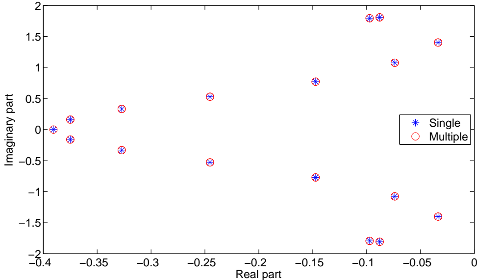
Figure 20: Spectrum of both the single and multi domain advection operator with \sigma = -1 and scaled with \Delta x , using 17 grid points for the 4th order accurate single domain operator and 34 for the multi domain operator. The multi domain operator spectrum is identical to the single domain operator spectrum since all eigenvalues of the multi domain operator are double eigenvalues.
