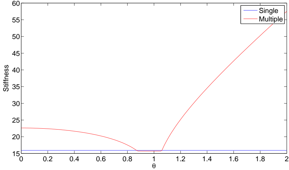
Figure 14: \max(\text{abs}(\lambda)) as function of \theta . The single domain operator is using 33 grid points and the multi domain operator is using 34 grid points.
