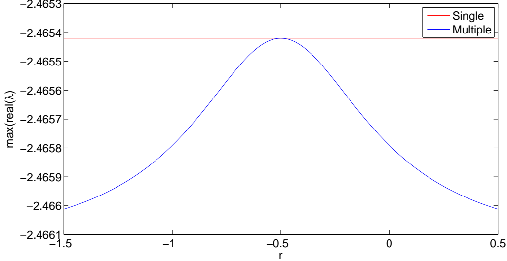
Figure 6: \max(\mathbb{R}(\lambda)) as a function of r . The single domain operator is using 33 grid points and the multi domain operator is using 34 grid points.
