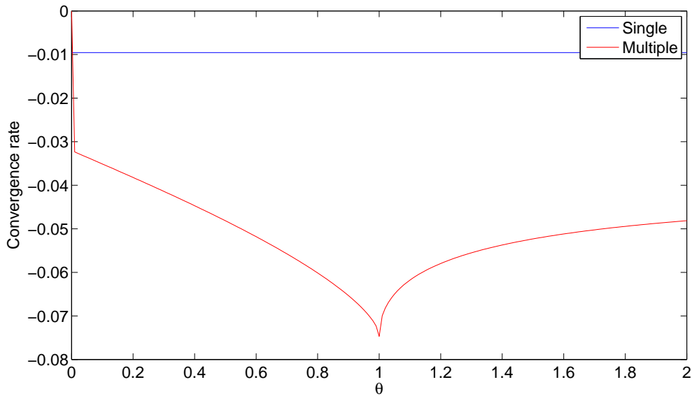
Figure 15: \max(\Re(\lambda)) as a function of \theta . The single domain operator is using 33 grid points and the multi domain operator is using 34 grid points.
