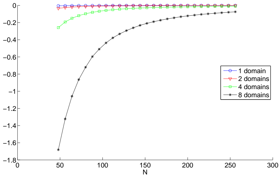
Figure 16: \max(\mathbb{R}(\lambda)) as a function of N with \theta = 1 .
