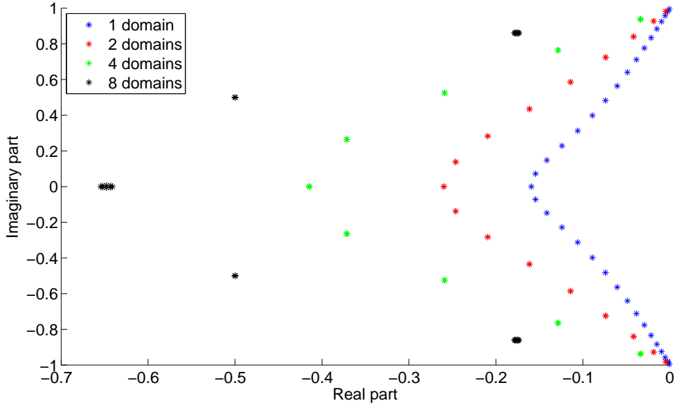
Figure 17: Spectra of the 1-, 2-, 4- and 8-domain operator scaled with \Delta x for \theta = 1 . Note that the eigenvalues of the 8-domain operator are clustered.
