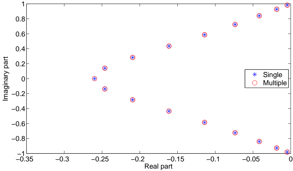
Figure 11: Spectrum of both the single and multi domain operator with \sigma = -1 and scaled with \Delta x , using 17 grid points for the single domain operator and 34 for the multi domain operator. The multi domain operator spectrum is identical to the single domain operator spectrum since all eigenvalues of the multi domain operator are double eigenvalues.
