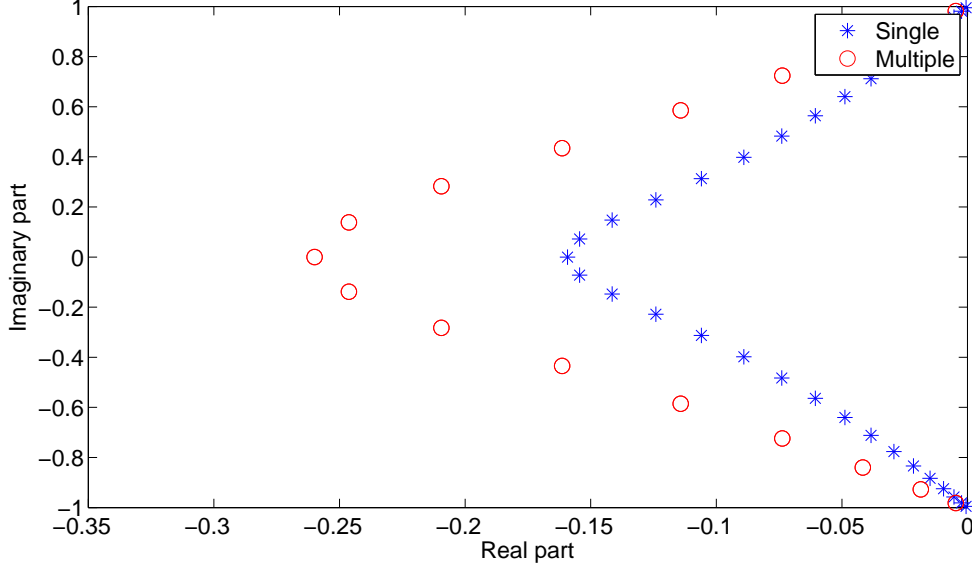
Figure 12: Spectrum of both the single and multi domain operator with \sigma = -1 and scaled with \Delta x using 33 grid points for the single domain operator and 34 for the multi domain operator
