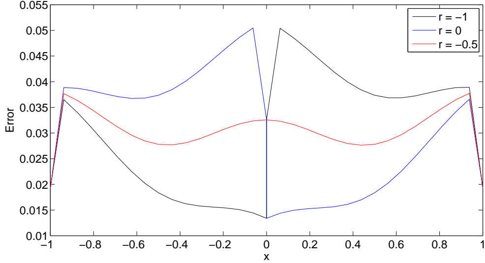
Figure 8: Difference at t = \frac{\pi}{2} between the analytic and computed solution with 34 grid points for different values of r
