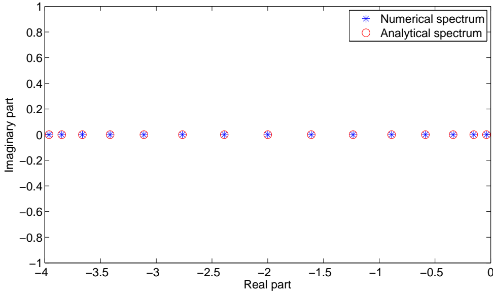
Figure 1: Analytical and computed numerical spectrum. There is a tripple root at \tilde{s} = -2 .
