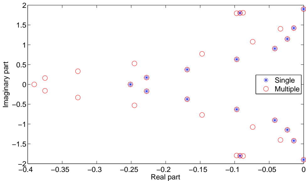
Figure 19: Spectrum of both the single and multi domain advection operator with \sigma = -\frac{1}{2} and scaled with \Delta x , using 17 grid points for the 4th order accurate single domain operator and 34 for the multi domain operator. The single domain operator spectrum is contained in the multi domain operator spectrum.
