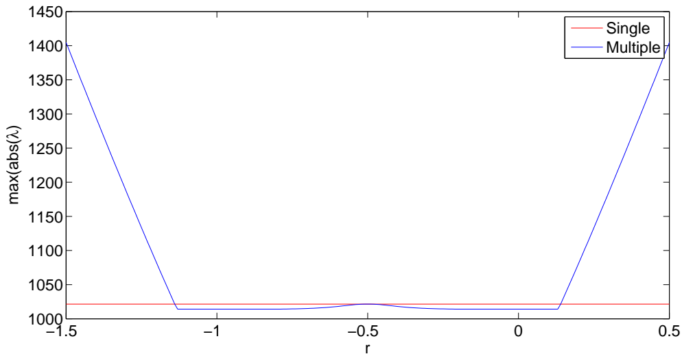
Figure 5: \max(\text{abs}(\lambda)) as function of r . The single domain operator is using 33 grid points and the multi domain operator is using 34 grid points.
