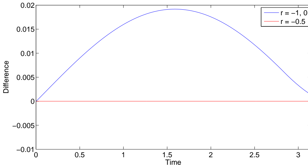
Figure 7: l_\infty -difference in time between the coupled and uncoupled solutions for different values of r with 33 grid points for the single domain and 34 for the multi domain.
