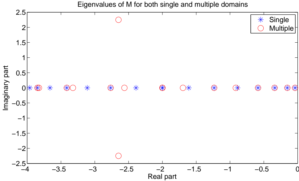
Figure 3: Eigenvalues of the single domain operator with 17 grid points and the multi domain operator with 18 grid points scaled with \Delta x^2 . r = 0 . All eigenvalues are identical if using r = -1 .
