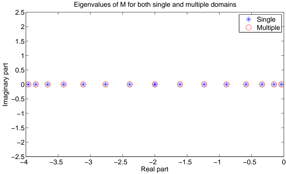
Figure 4: Eigenvalues of the single domain operator with 17 grid points and the multi domain operator with 18 grid points scaled with \Delta x^2 . r = -\frac{1}{2} .
