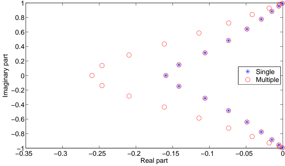
Figure 10: Spectrum of both the single and multi domain operator with \sigma = -\frac{1}{2} and scaled with \Delta x , using 17 grid points for the single domain operator and 34 for the multi domain operator. The single domain operator spectrum is contained in the multi domain operator spectrum.
