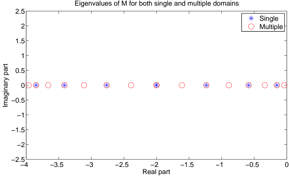
Figure 2: Eigenvalues of the single domain operator with 9 grid points and the multi domain operator with 18 grid points scaled with \Delta x^2 . The single domain operator spectrum is always contained in the multi domain operator spectrum independent of the interface parameter r . There is a tripple root at \tilde{s} = -2 .
