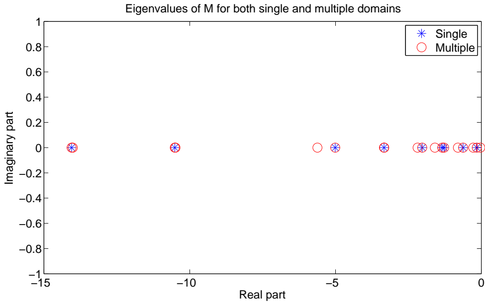
Figure 18: Eigenvalues of the 4th order accurate single domain diffusion operator with 9 grid points and the multi domain operator with 18 grid points scaled with \Delta x^2 . The single domain operator spectrum is always contained in the multi domain operator spectrum independent of the interface parameter r . Here r = -\frac{1}{2} .
