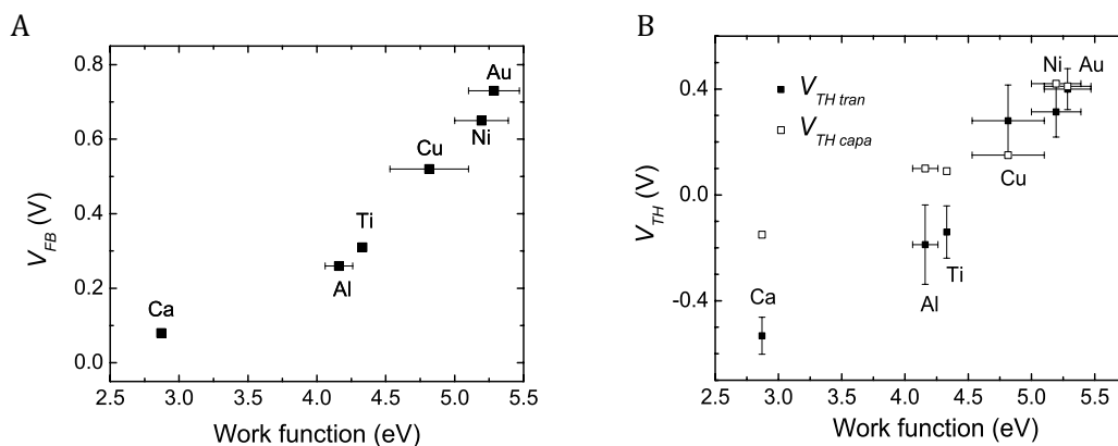
Fig. S3. Influence of the gate work function on (A) V_{FB} and (B) V_{TH} obtained from capacitance ( V_{TH\ capa} ) and transistor ( V_{TH\ tran} ) measurements.
