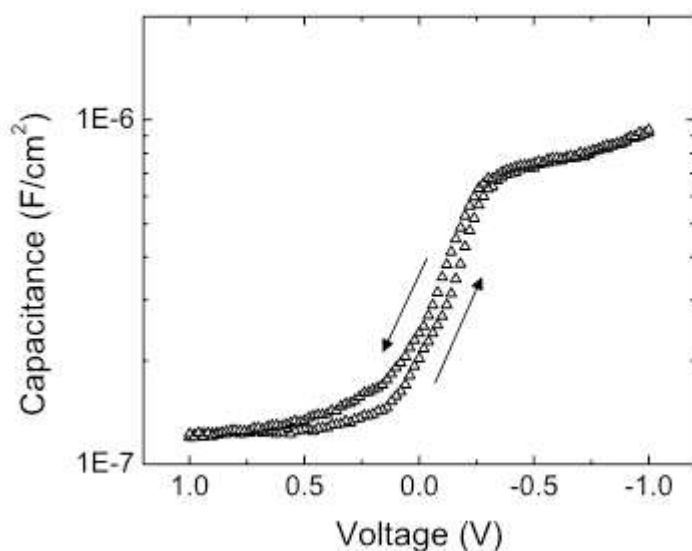
Fig. S1. Variation of the effective capacitance as a function of the voltage for a capacitor with a Ca top electrode. The capacitance is shown for a forward and backward voltage sweep.
