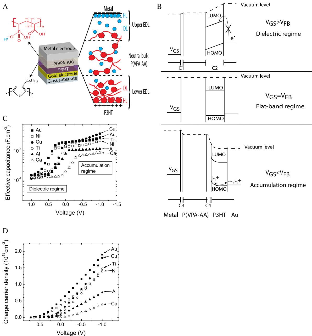
Fig. 1. Metal-Electrolyte-Semiconductor diode. (A) Schematic cross-section of the MES diode with the chemical formulae of P3HT and P(VPA-AA) and a schematic representation of charge distribution in the system capacitor. The red features represent the polyanionic chains and the blue circles the mobile protons. (B) Energy diagram of the different regimes of a metal-insulator-semiconductor stack. (C) Plot of the effective capacitance as a function of the voltage for six metals: Au (full squares), Ni (open squares), Cu (full circles), Ti (open circles), Al (full triangles) and Ca (open triangles). (D) Variation of the charge carrier density as a function of the gate voltage.
