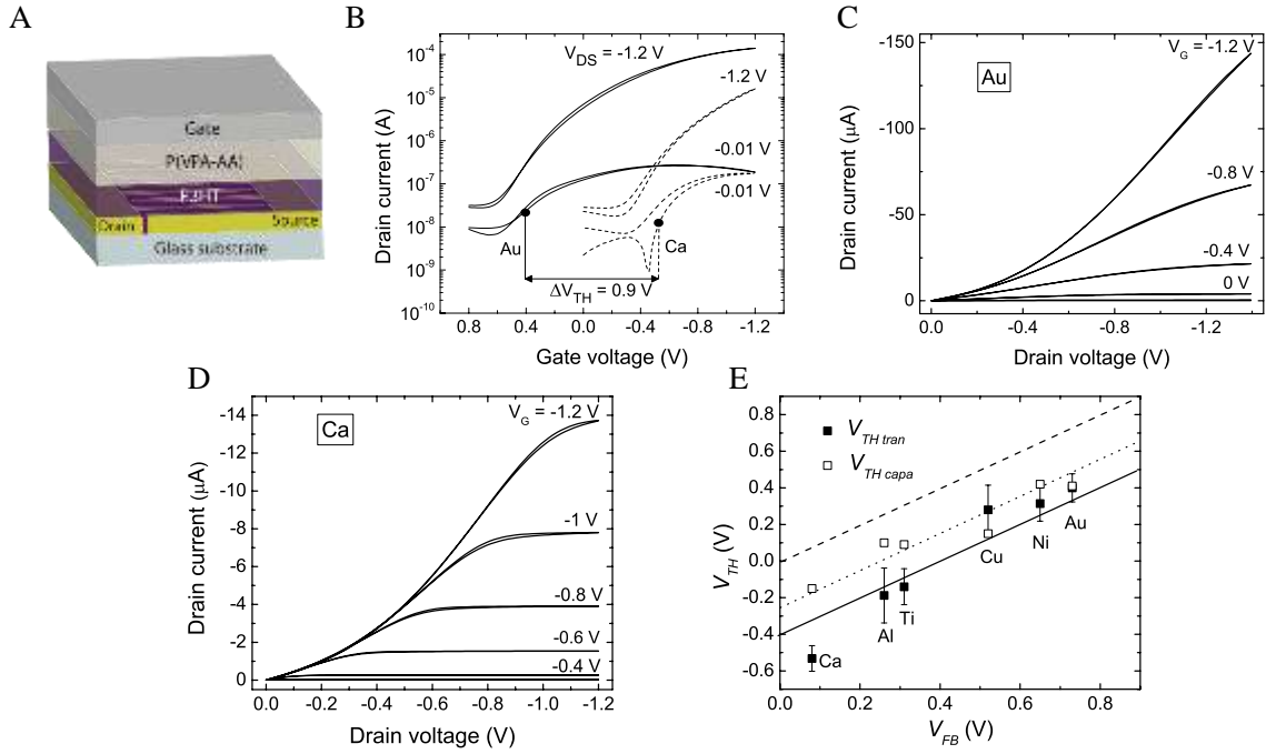
Fig. 2. Electrolyte-gated OFETs with various metals. (A) Schematic representation of the OFET. (B) Transfer characteristics, in the linear regime ( V_{DS} = -0.01 V) and at saturation ( V_{DS} = -1.2 V), for electrolyte-gated OFETs with Au (full line) and Ca (dashed line) as gate metal. Output characteristics for electrolyte-gated OFET with (C) Au and (D) Ca as gate metal. (E) Variation of the threshold voltage extracted from the capacitance, V_{TH\ capa} , (empty squares) and transistor measurements, V_{TH\ tran} , (full black squares) as a function of the flat-band potential. The dotted and full lines are linear fits with a slope of 1 to the data corresponding to capacitance and transistor measurements, respectively. The dashed line represents the ideal case where V_{TH} = V_{FB} .
