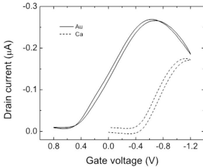
Fig. S2. Transfer curves at V_{DS} = 0.01 V for transistors with Au (full line) and Ca (dashed line) gates.
