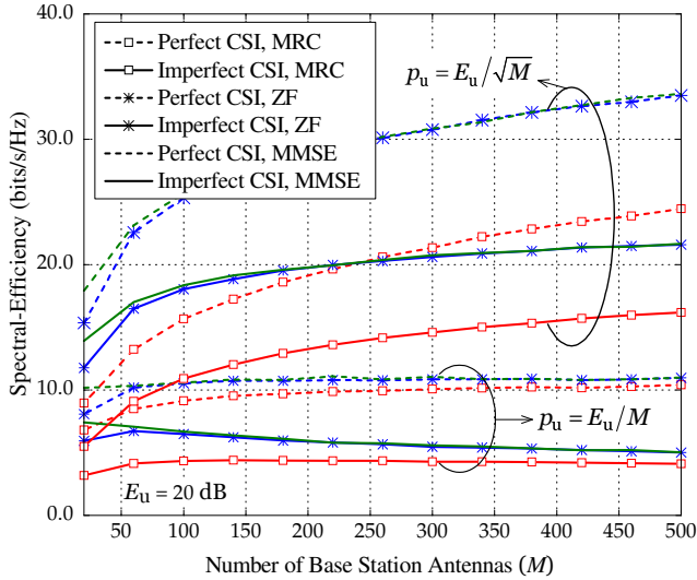
Fig. 2. Spectral efficiency versus the number of BS antennas M for MRC, ZF, and MMSE processing at the receiver, with perfect CSI and with imperfect CSI (obtained from uplink pilots). In this example K = 10 users are served simultaneously, the reference transmit power is E_u = 20 dB, and the propagation parameters were \sigma_{\text{shadow}} = 8 dB and \nu = 3.8 .
