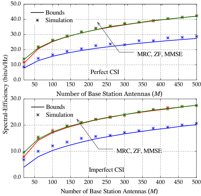
Fig. 1. Lower bounds and numerically evaluated values of the spectral efficiency for different numbers of BS antennas for MRC, ZF, and MMSE with perfect and imperfect CSI. In this example there are K = 10 users, the coherence interval T = 196 , the transmit power per terminal is p_u = 10 dB, and the propagation channel parameters were \sigma_{\text{shadow}} = 8 dB, and \nu = 3.8 .
