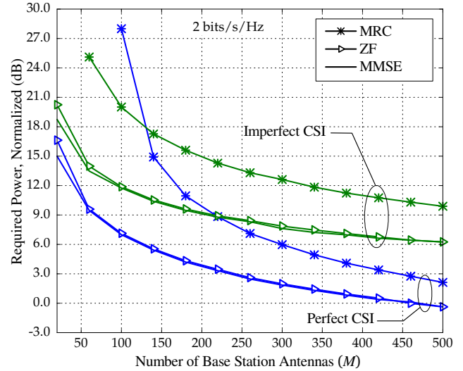
Fig. 5. Same as Figure 4 but for a target spectral efficiency of 2 bits/channel use per user.
