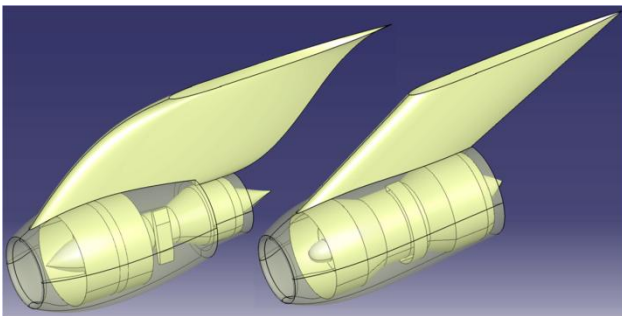
Fig. 12: Turbofan with trapezoidal gearbox, separate jet nacelle and smooth leading/trailing edge nacelle (left) and turbojet engine with circular gearbox, mixed flow nacelle and straight leading/trailing edge pylon (right)
