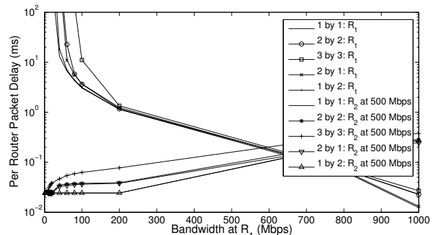
Figure 5: The 99-percentile per-router packet delays for each of the two routers ( R_1 and R_2 ), under different link rates (shown on x-axis for R_1 and in the label for R_2 ) and scenarios (label).
