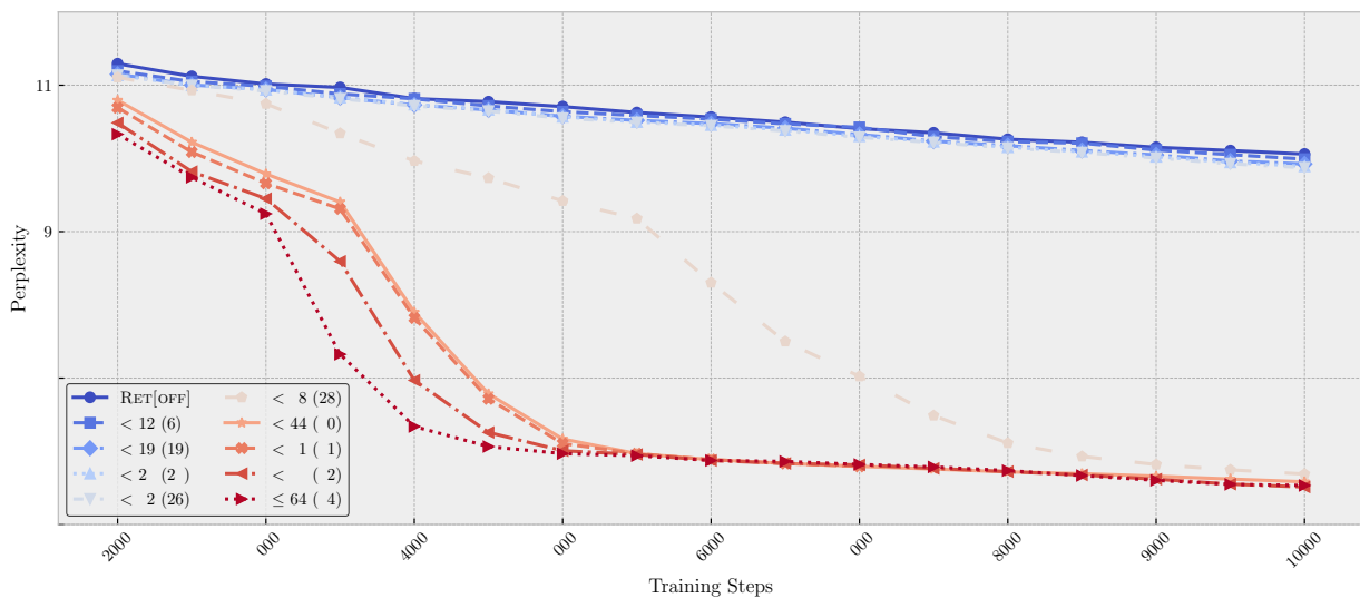
Figure 2: Test perplexity trends for models with different overlap thresholds over training steps. The colors, as well as the line and dot styles, represent the threshold, with colors going from cold to warm as the threshold increases. The legend shows the threshold value, followed by the average overlap for that experiment in parentheses.
