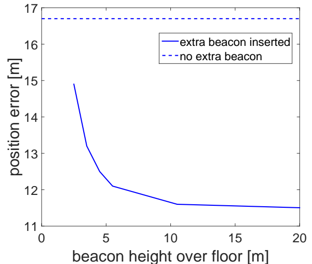
Fig. 13: An illustration of how the positioning accuracy in the z -direction is increased when an additional beacon, centered in the middle of the original beacons but at varying height, is introduced. The dashed line corresponds to the error from Section IV-B1 with the original setup and the solid lines corresponds to the error when the additional beacon is introduced.
